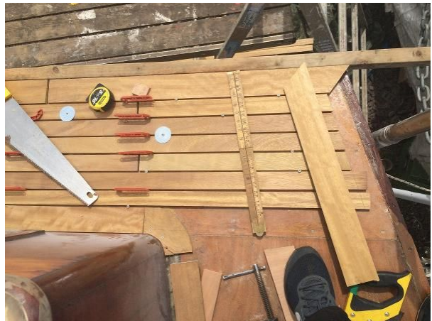
Wooden Motor Yacht decks being relaid
